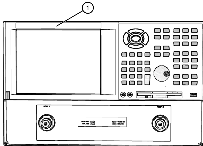
Figure 1 Nameplate Replacement
